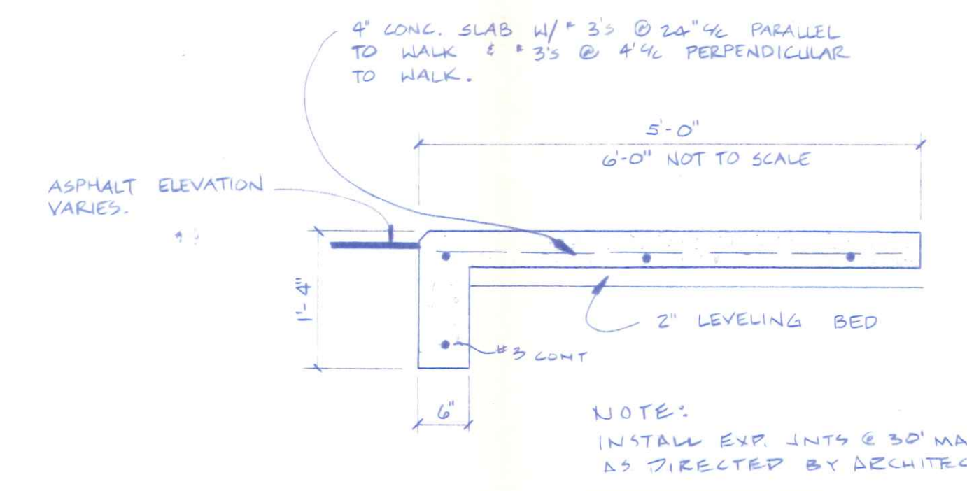
WALK DETAIL SCALE: 3/4"=1'-0"
